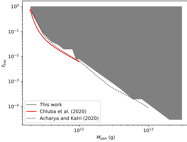
Figure 1: CMB spectral distortions constraints on PBH mass M_{\text{PBH}} and PBH - dark matter density fraction f_{\text{frac}} . The gray region shows forbidden values of M_{\text{PBH}} and f_{\text{frac}} due to the experimental limit \delta I/I = 5 \times 10^{-5} set by the COBE-FIRAS data in Fixsen et al. (1996).
