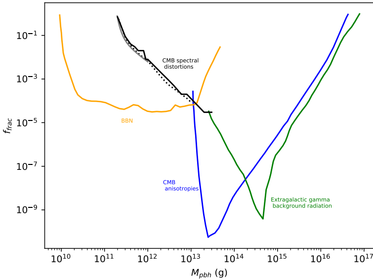
Figure 2: Constraints on PBH mass M_{\text{PBH}} and PBH - dark matter density fraction f_{\text{frac}} due to different cosmological observables. The region above the curves is prohibited. The big bang nucleosynthesis constraints are due to Carr et al. (2010), CMB anisotropies constraints are due to Acharya and Khatri (2020a), extragalactic gamma background radiation constraints are due to Carr et al. (2010), for the CMB spectral distortions constraints, the black dotted line shows those found in Acharya and Khatri (2020b), the solid gray line shows those found in Chluba et al. (2020). The solid black line shows the constraints obtained in this work.
